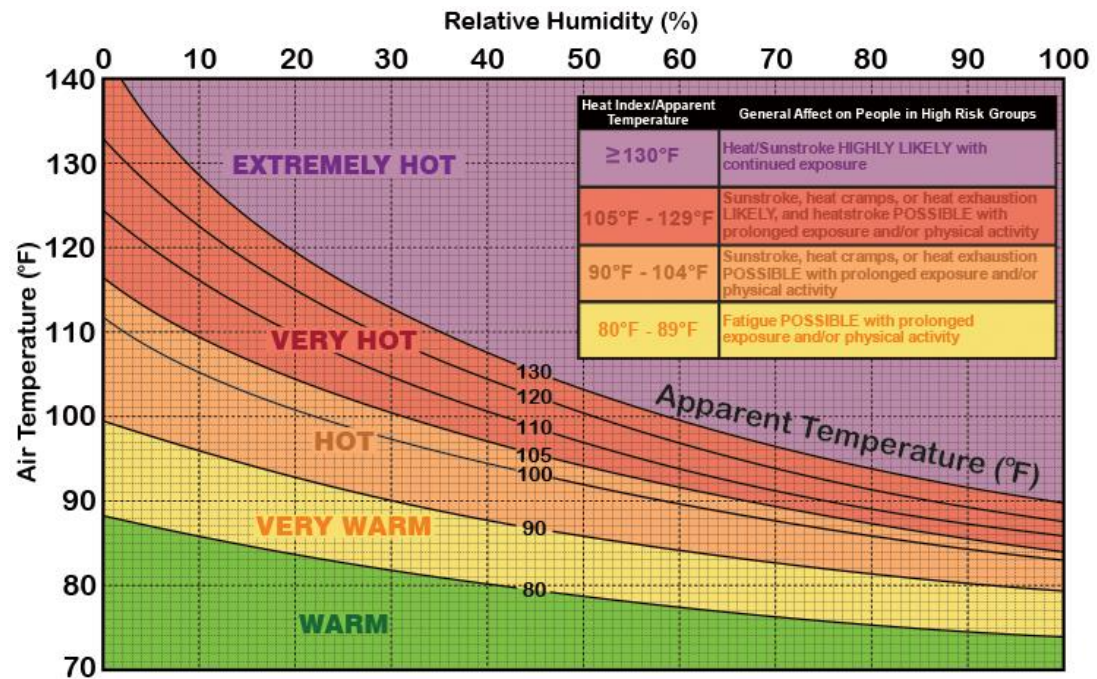
Figure 22 Heat Index
