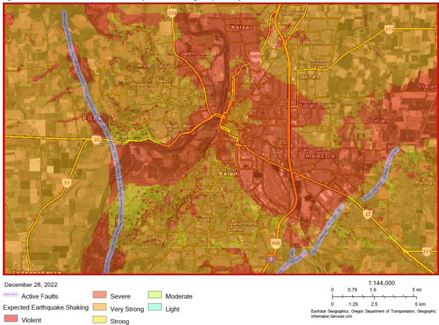
Figure 15 Cascadia Subduction Zone Expected Shaking Map of City of Salem
