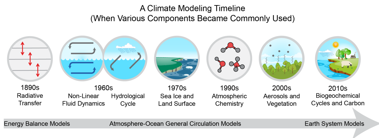
Figure 1. As scientific understanding of climate has evolved over the last 120 years, increasing amounts of physics, chemistry, and biology have been incorporated into calculations and, eventually, models. Various processes and components of the climate system became regularly included in scientific understanding of global climate calculations and, over the second half of the century as computing resources became available, formalized in global climate models. (Source: science2017.globalchange.gov )
