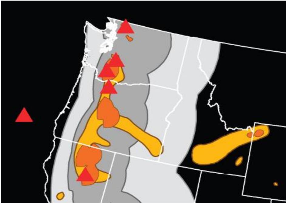
Figure 38 National Volcanic Hazard Map
