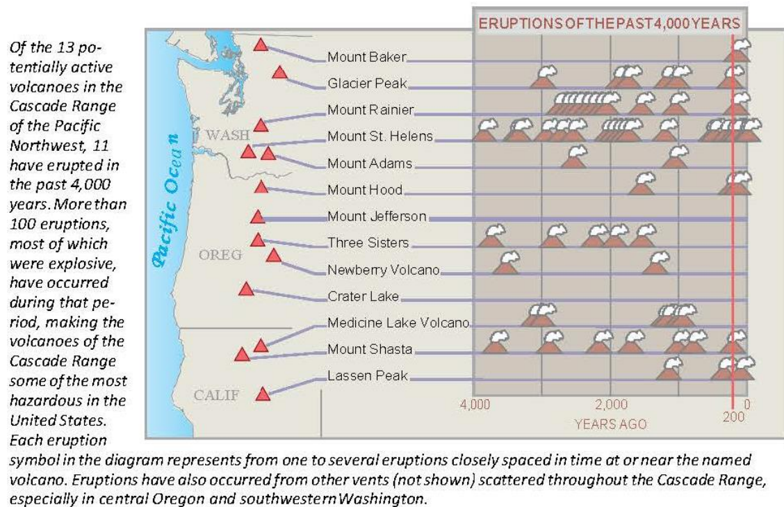
Figure 40 Potentially Active Volcanoes in the Western United States
