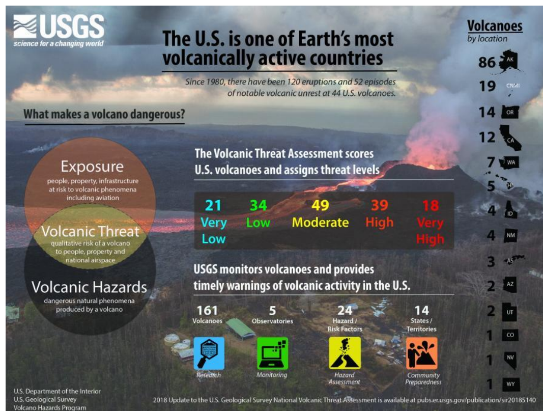
Figure 39 Volcanic Threat Assessment Statistics
