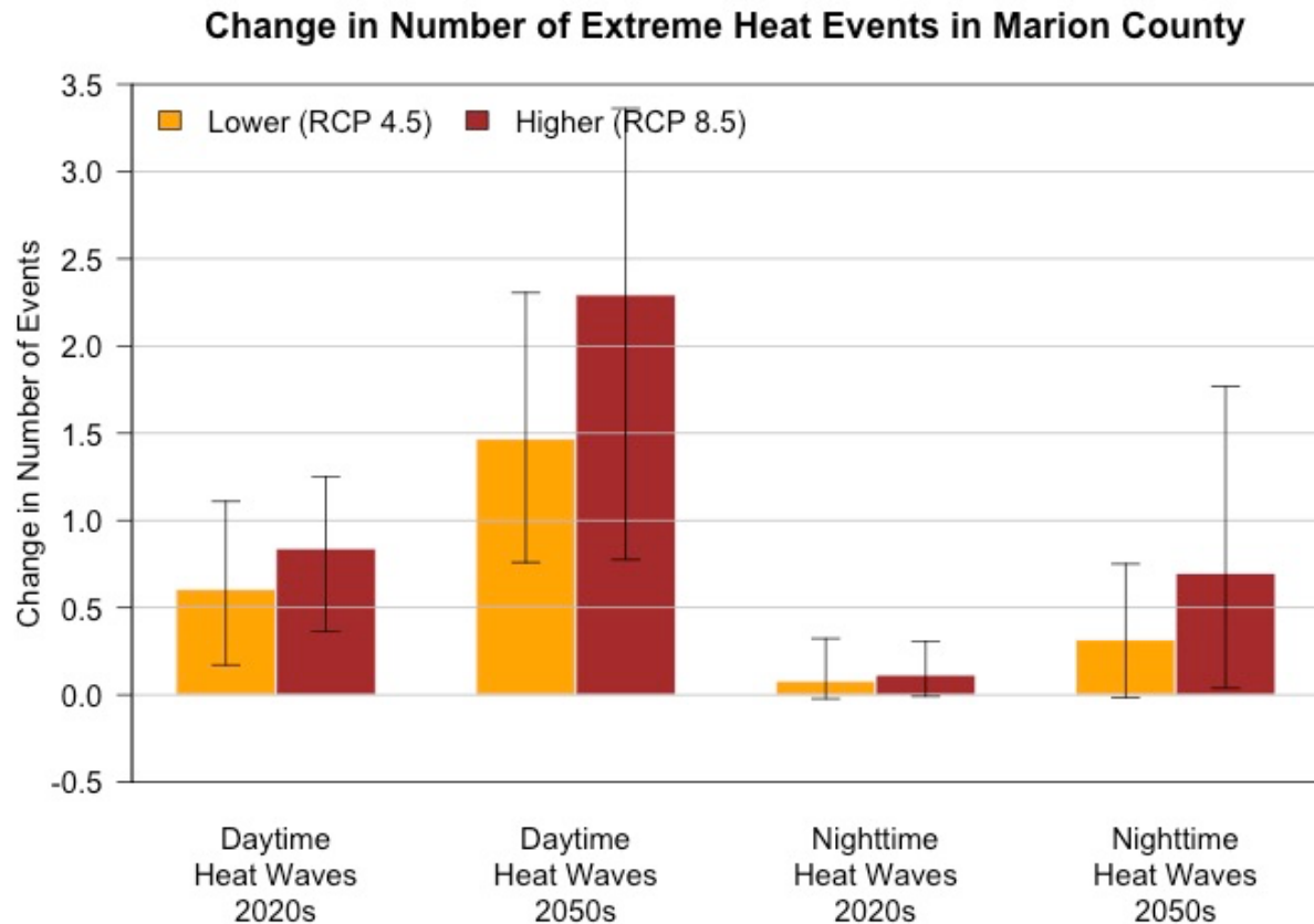
Figure 6. Projected changes in the number of daytime heat waves (left two sets of bars) and nighttime heat waves (right two sets of bars) in Marion County by the 2020s (2010–2039 average) and 2050s (2040–2069 average), relative to the historical baseline (1971–2000 average), under two emissions scenarios. Changes were calculated for each of 20 global climate models relative to each model’s historical baseline, then averaged across the 20 models. Whiskers represent the range of changes across 20 models. Daytime heat waves are defined as three or more consecutive days on which the maximum temperature is 90°F or higher; nighttime heat waves are three or more consecutive days on which the minimum temperature is 65°F or higher.
