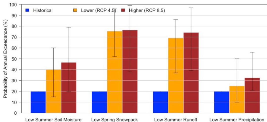
Figure 14 Projected Future Drought in Marion County
