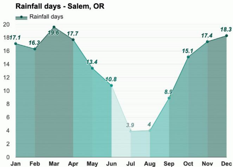
Figure C-3 Average Monthly Rainfall Days, Salem, Oregon
