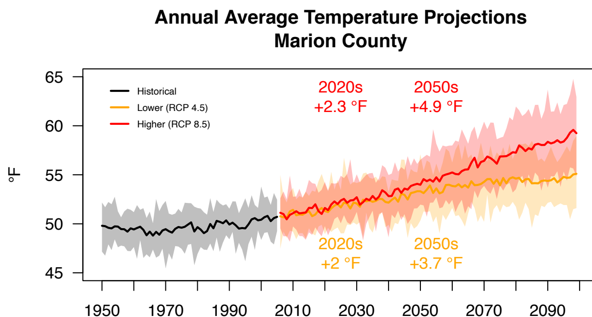
Figure 3. Projected annual average temperature in Marion County as simulated by 20 downscaled global climate models under a lower (RCP 4.5) and a higher (RCP 8.5) greenhouse gas emissions scenario. Solid lines and shading represent the 20-model mean and range, respectively. The figure shows the multiple-model mean differences for the 2020s (2010–2039 average) and the 2050s (2040–2069 average) relative to the average historical baseline (1971–2000 average).
