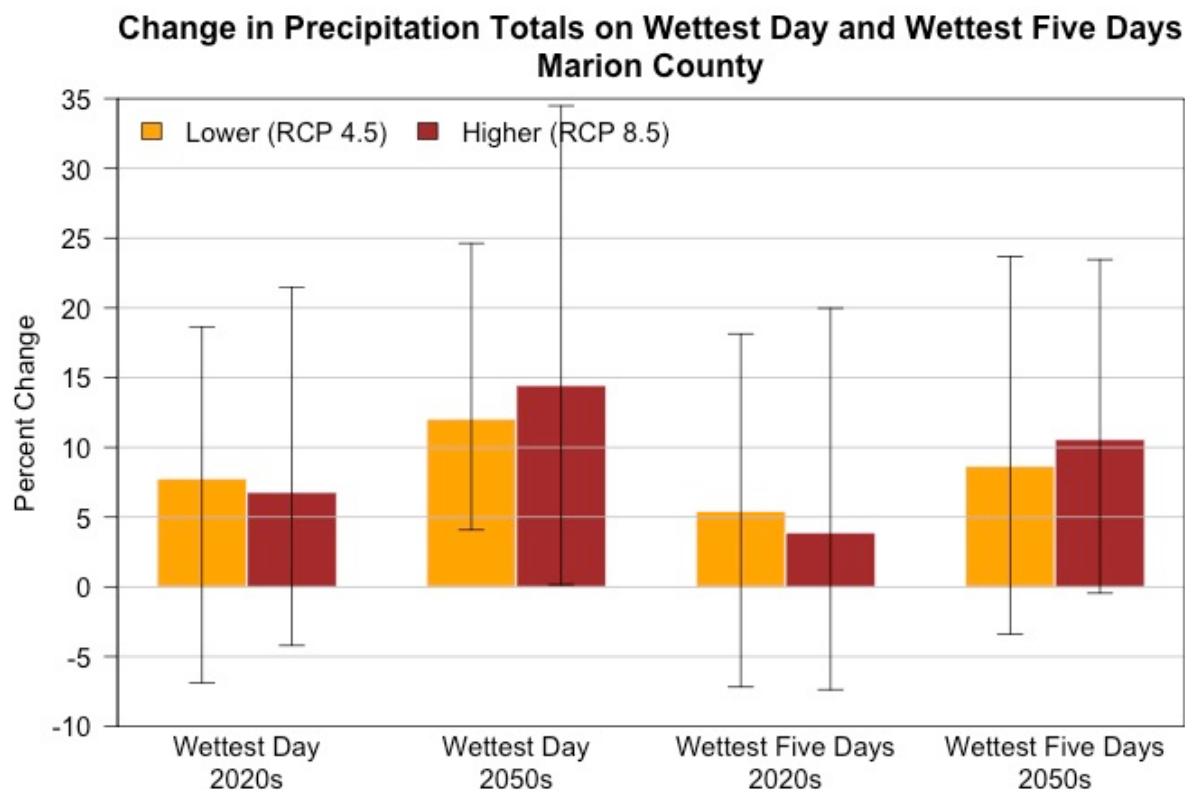
Figure 10. Projected percent changes in the amount of precipitation on the wettest day of the year (left two sets of bars) and wettest consecutive five days of the year (right two sets of bars) in Marion County by the 2020s (2010–2039 average) and 2050s (2040–2069 average), relative to the historical baseline (1971–2000 average), under two emissions scenarios. Changes were calculated for each of 20 global climate models relative to each model’s historical baseline, then averaged across the 20 models. Whiskers represent the range of changes across 20 models.
