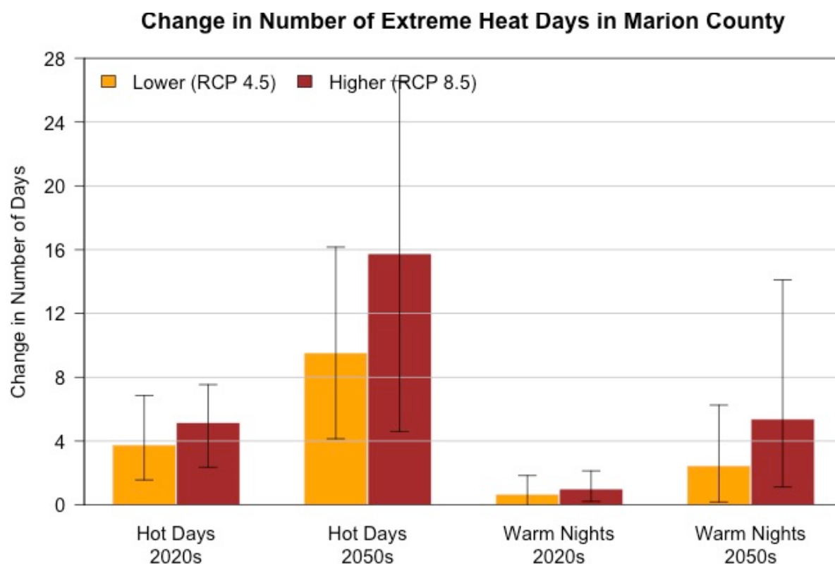
Figure 4. Projected changes in the number of hot days (left two sets of bars) and warm nights (right two sets of bars) in Marion County by the 2020s (2010–2039 average) and 2050s (2040–2069 average), relative to the historical baseline (1971–2000 average), under two emissions scenarios. Changes were calculated for each of 20 global climate models relative to each model’s historical baseline, then averaged across the 20 models. Whiskers represent the range of changes across 20 models. Hot days are those on which the maximum temperature is 90°F or higher; warm nights are those on which the minimum temperature is 65°F or higher.
