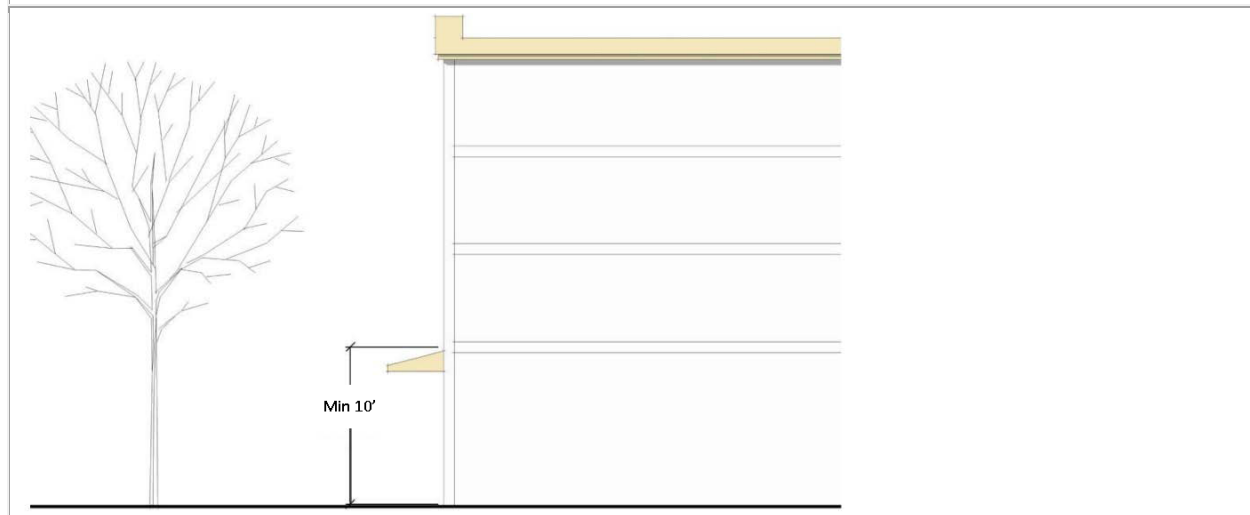
FIGURE 536-2 GROUND FLOOR HEIGHT
