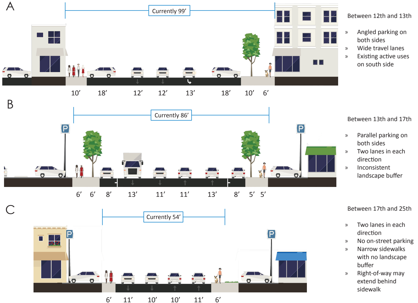
Figure 4. State Street- Existing Cross Sections
