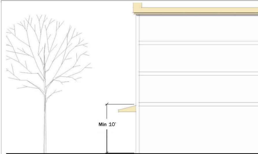
FIGURE 534-1 GROUND FLOOR HEIGHT
